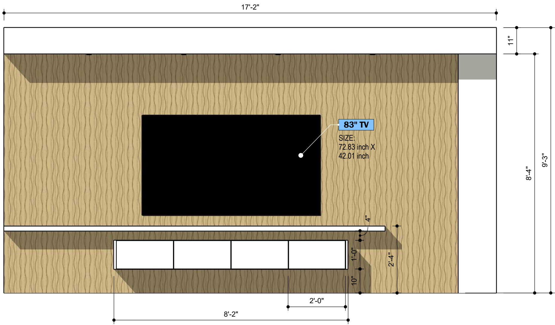
FRONT VIEW Scale 1:24
