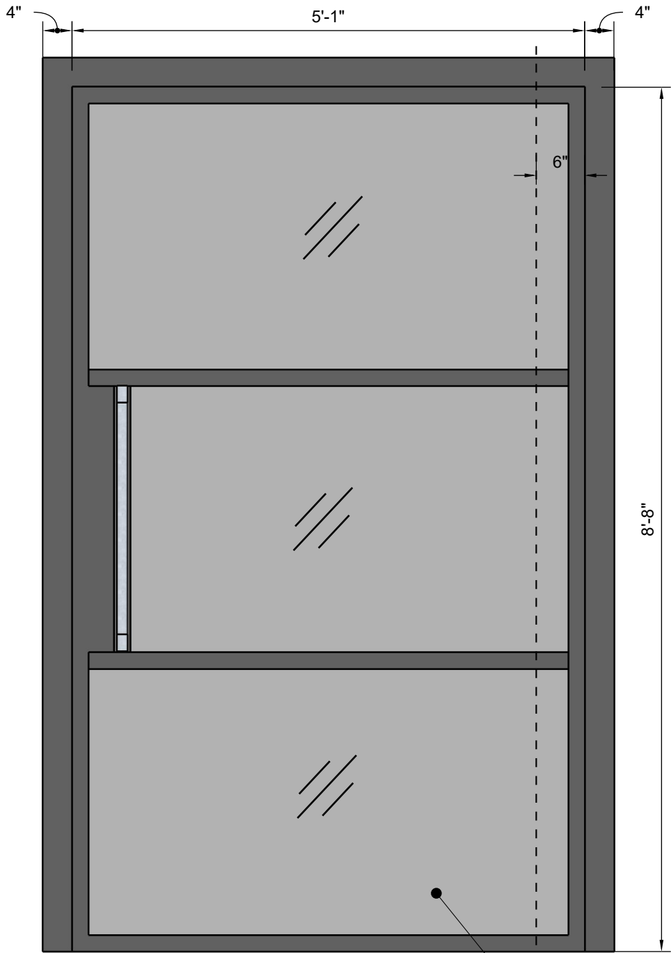
FRONT VIEW Scale 1:16
