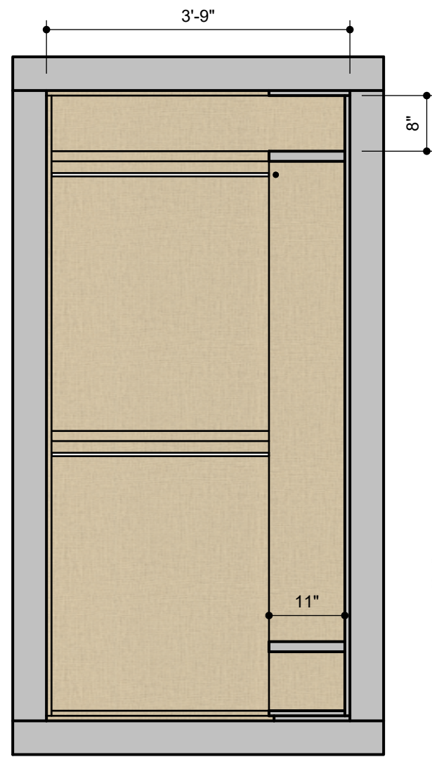
SECTION A
