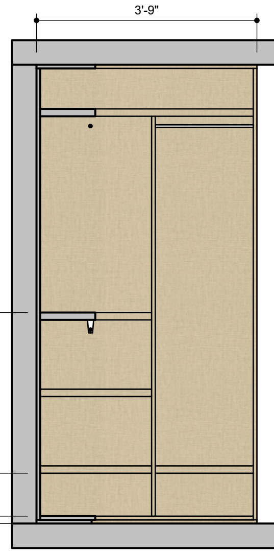
SECTION B
