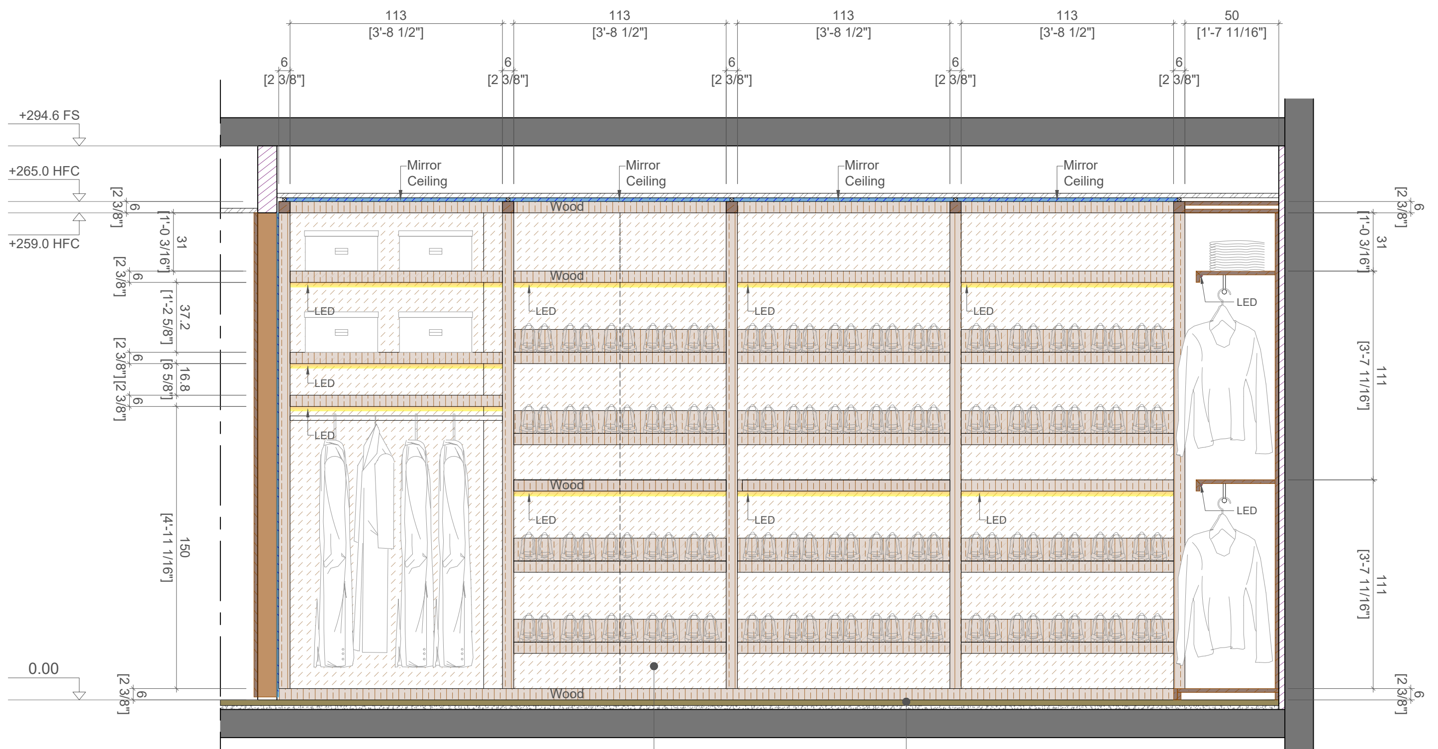
ELEVATION AA
