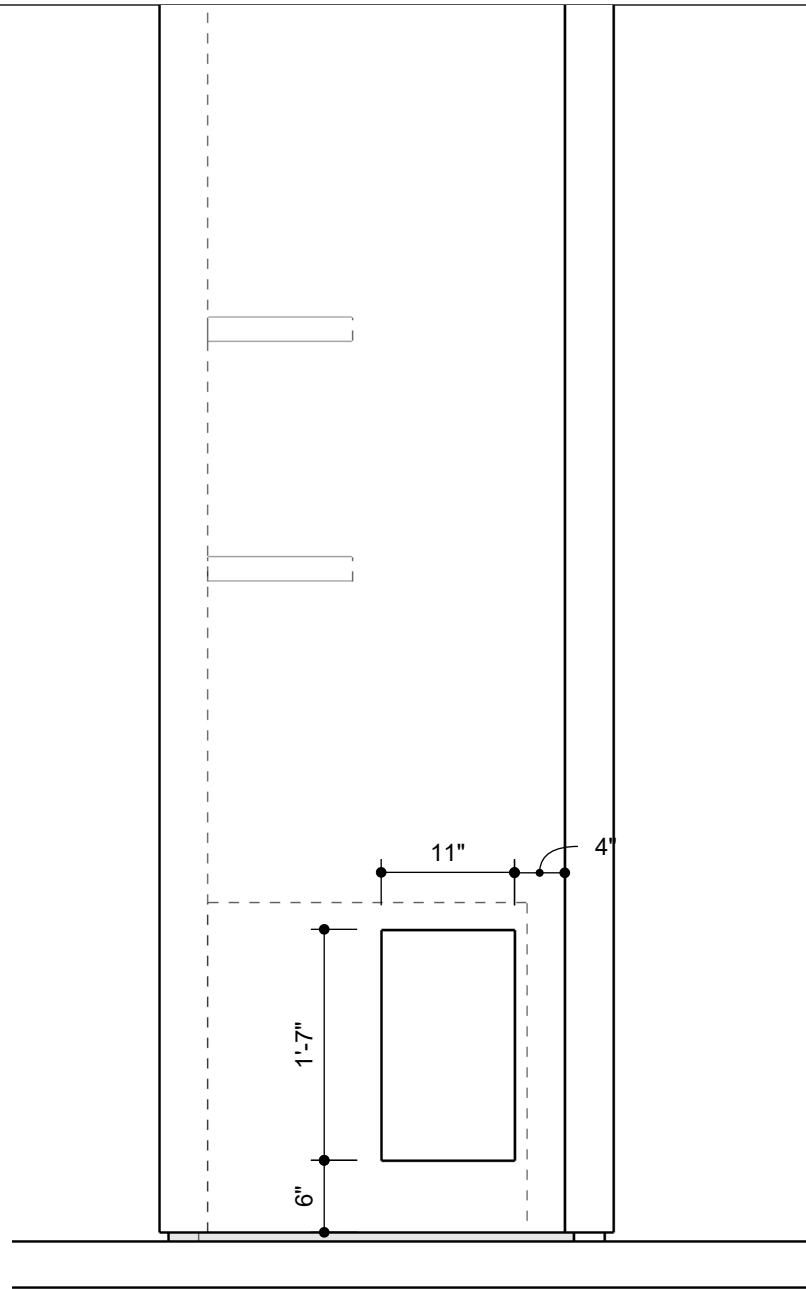
PARTITION HOLE FRONT VIEW
