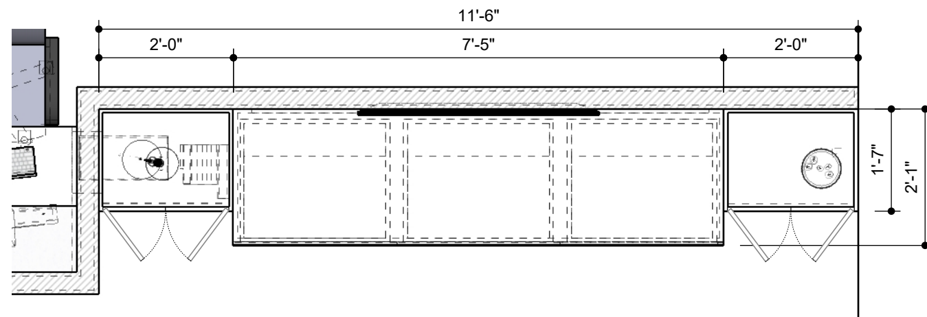
TOP VIEW Scale 1:16
