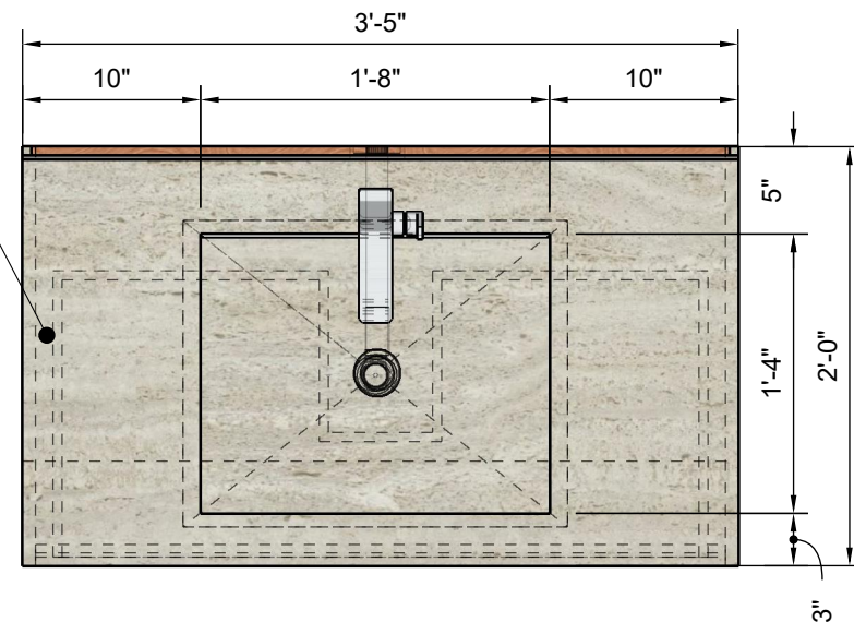
TOP VIEW Scale 1:16
