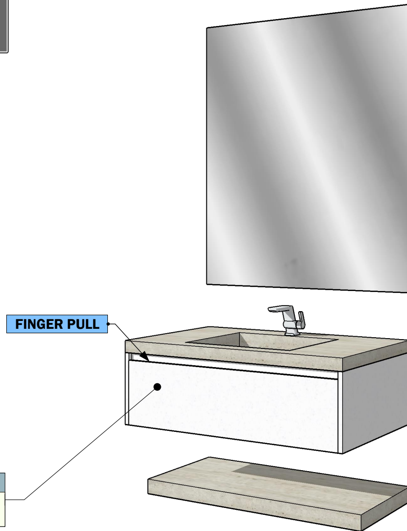
PERSPECTIVE VIEW Not Scaled
