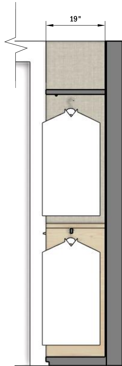
SECTION A Scale 1:16
