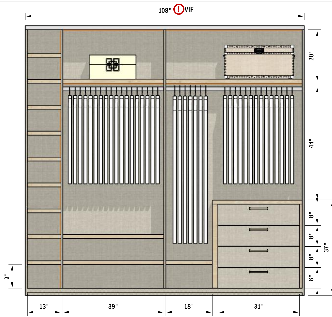
FRONT VIEW Scale 1:16
