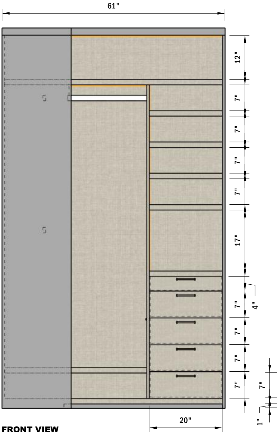
FRONT VIEW Scale 1:16
