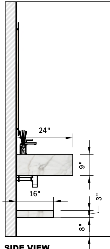
SIDE VIEW Scale 1:24
