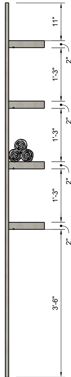
SIDE VIEW
