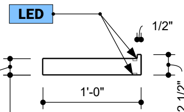
FRONT VIEW Scale 1:16
