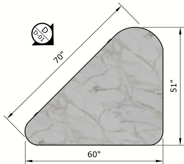
TOP VIEW Scale 1:24
