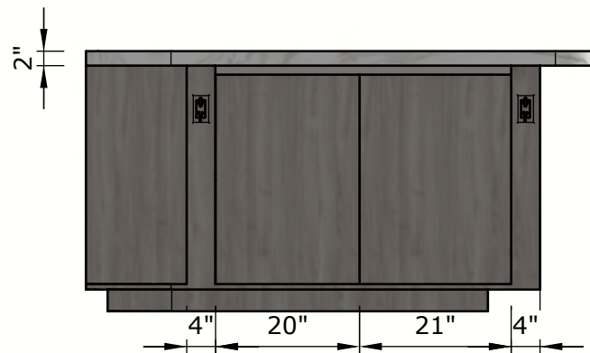
VIEW D Scale 1:24
