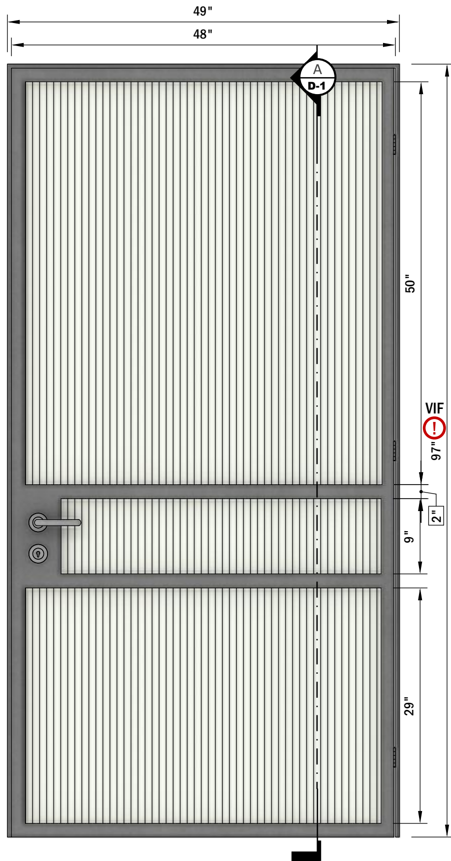
FRONT VIEW
