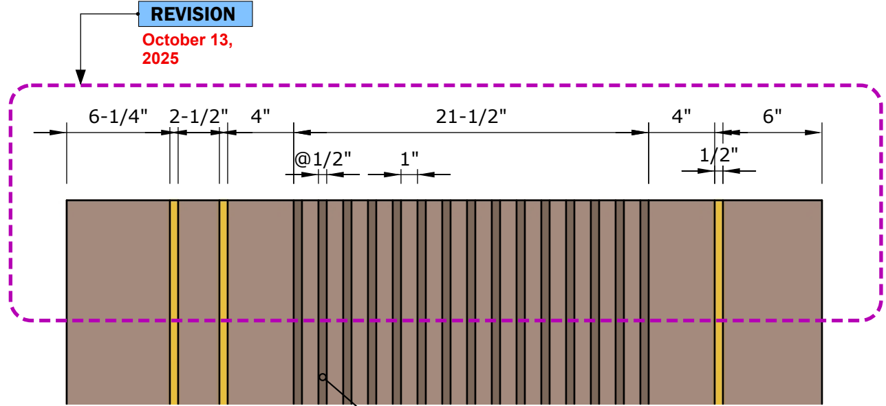
DETAIL A Scale 1:8
