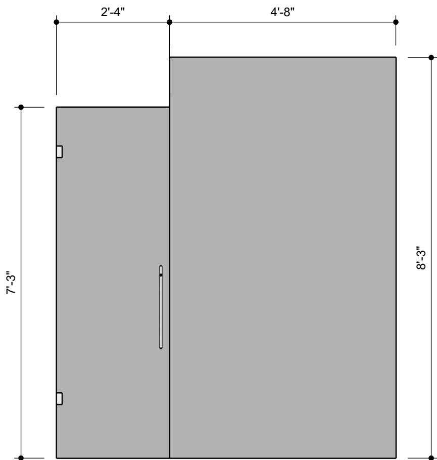
MASTER SHOWER ENCLOSURE A FRONT VIEW Scale 1:24
