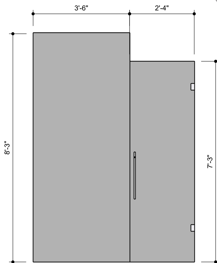
BATH. No 2 SHOWER ENCLOSURE B FRONT VIEW Scale 1:24
